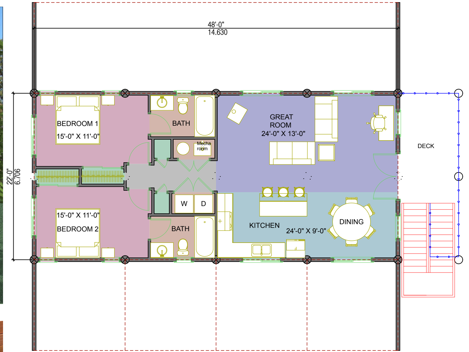
SECOND FLOOR PLAN AREA: 1056 SQ. FT. 98 SQ.M.
